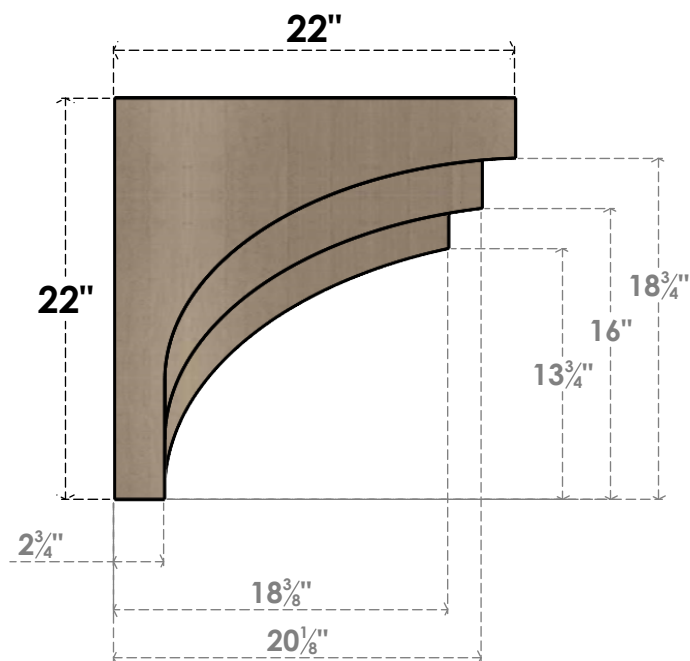
SIDE PROFILE
