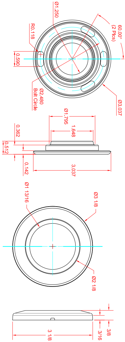
IFSS-CER-FLANGE Detail
