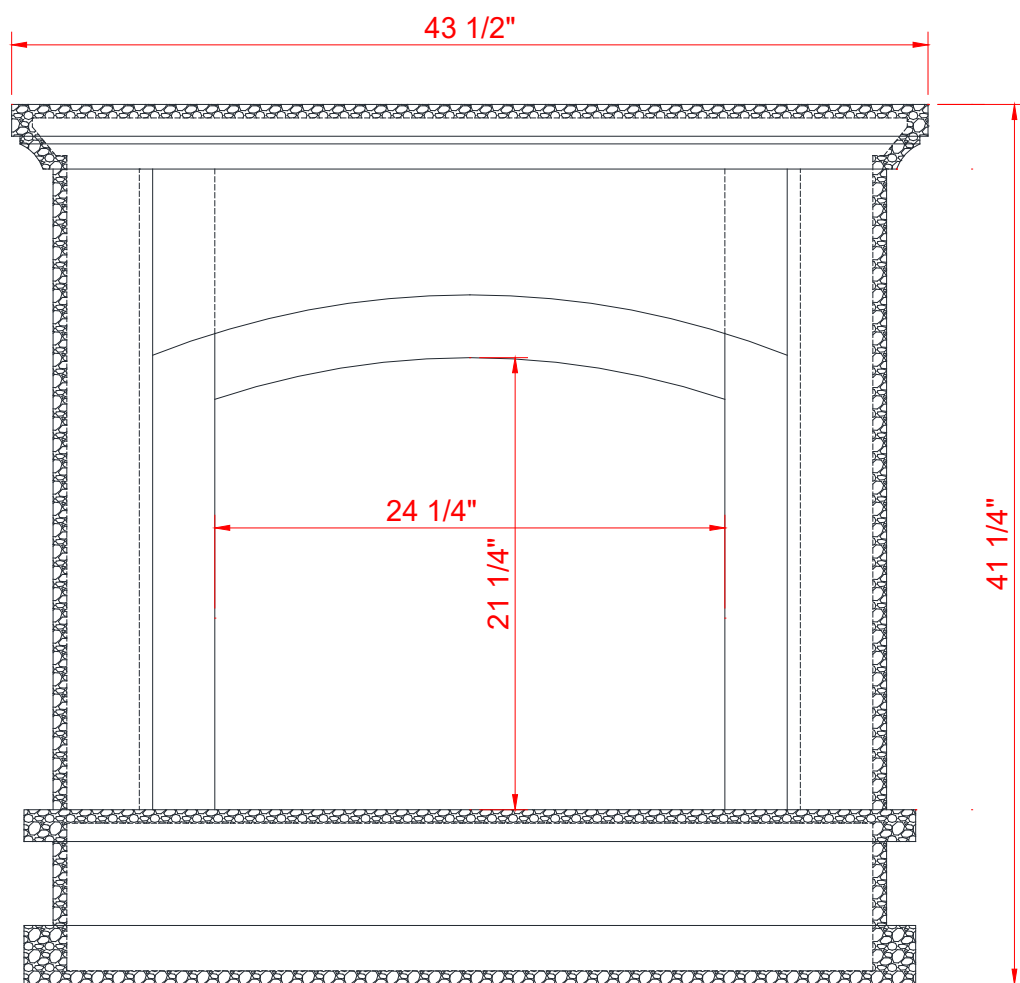
FRONT VIEW
