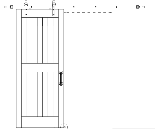
Our preferred location of the floor guide
