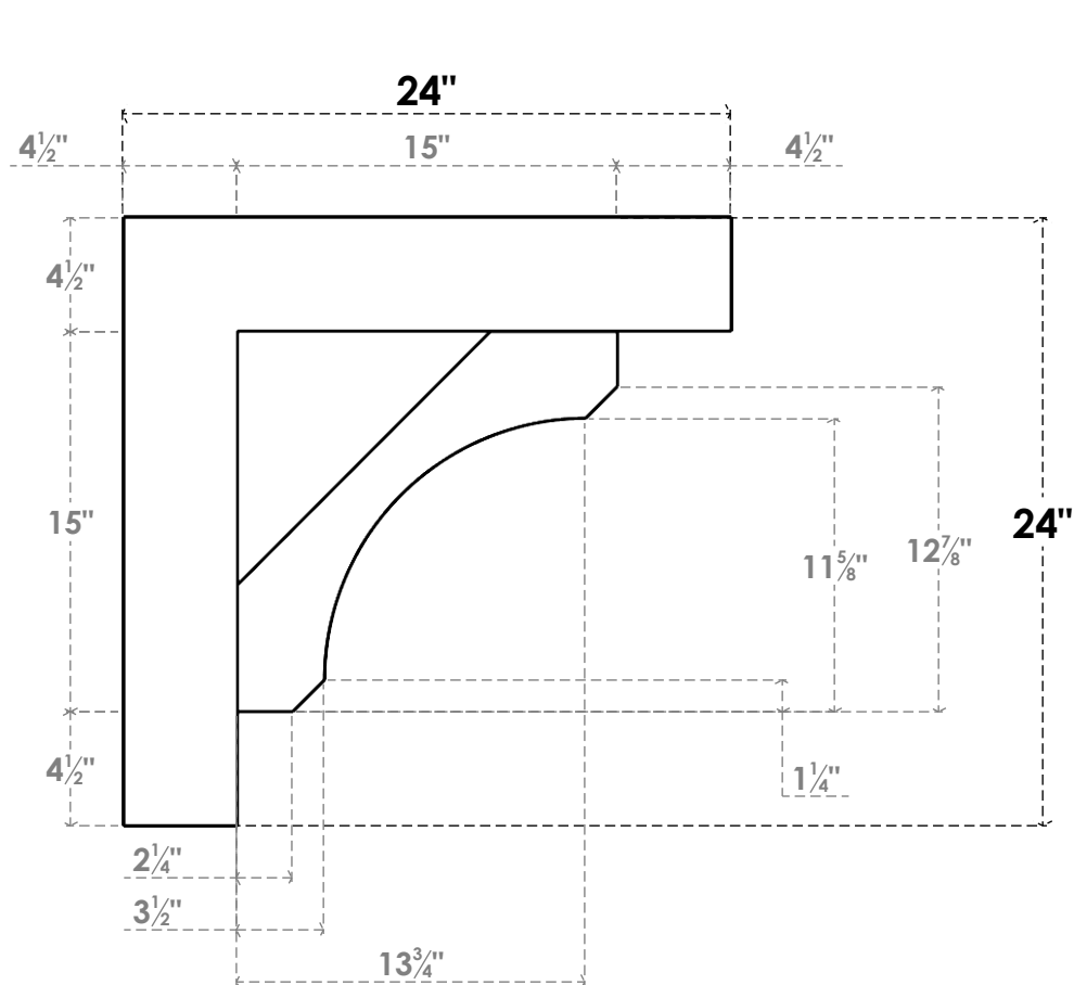
SIDE PROFILE
