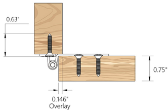
Cross section
