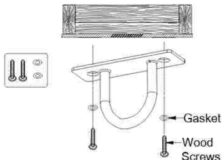
Ceiling Joist
