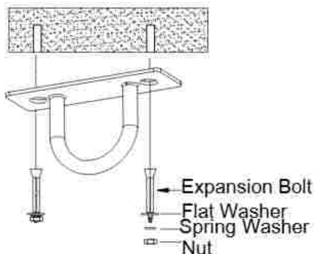
Concrete Ceiling
