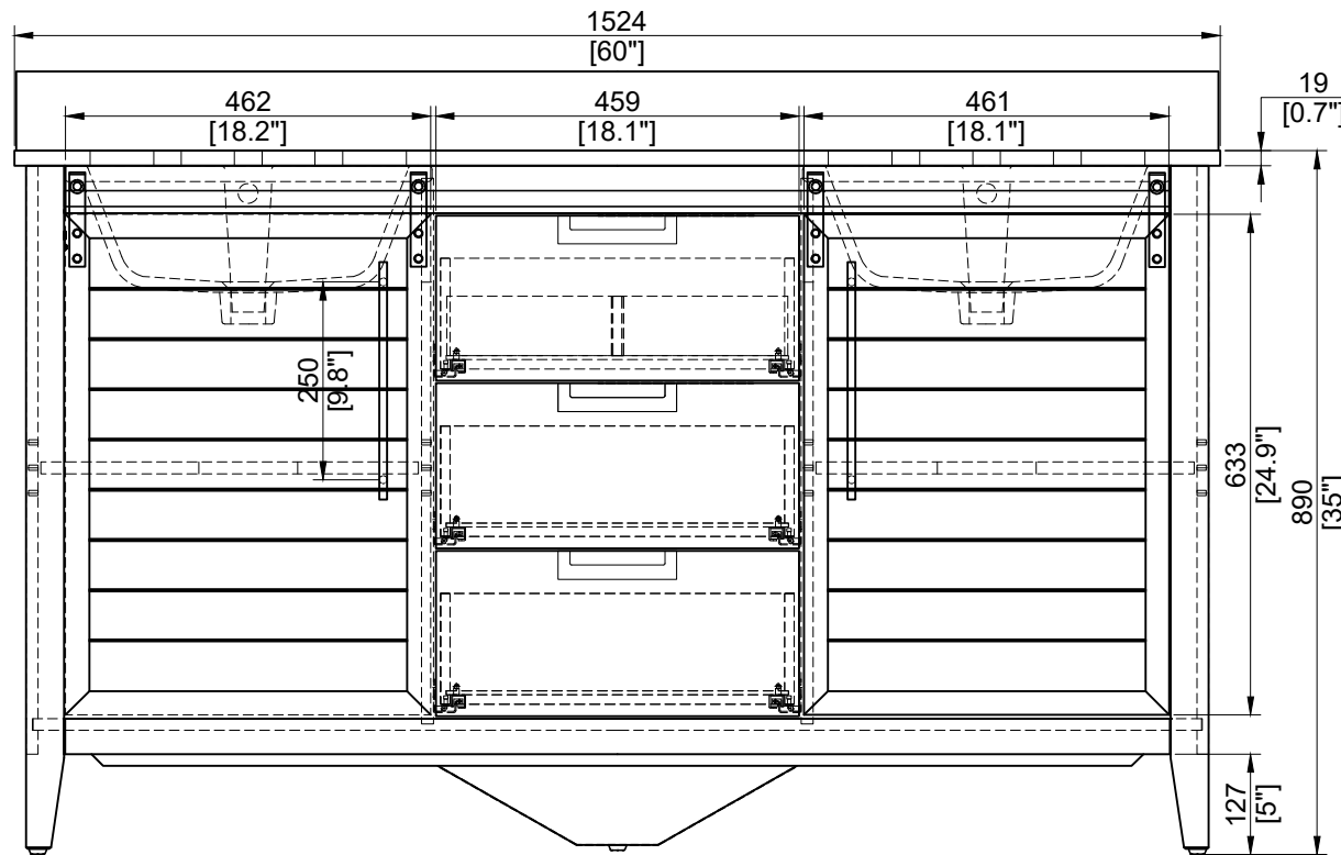
FRONT VIEW
