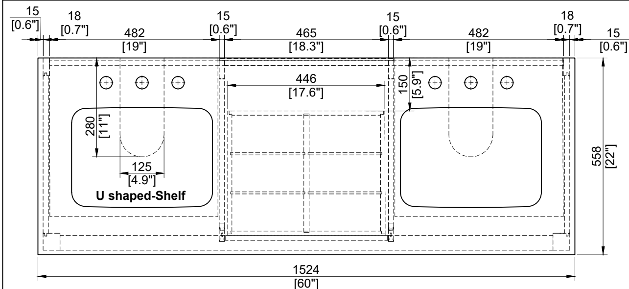
DETAIL VIEW
