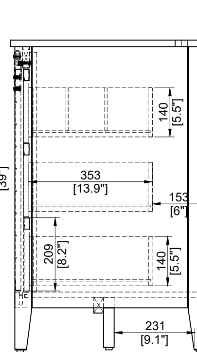
SIDE VIEW 2
