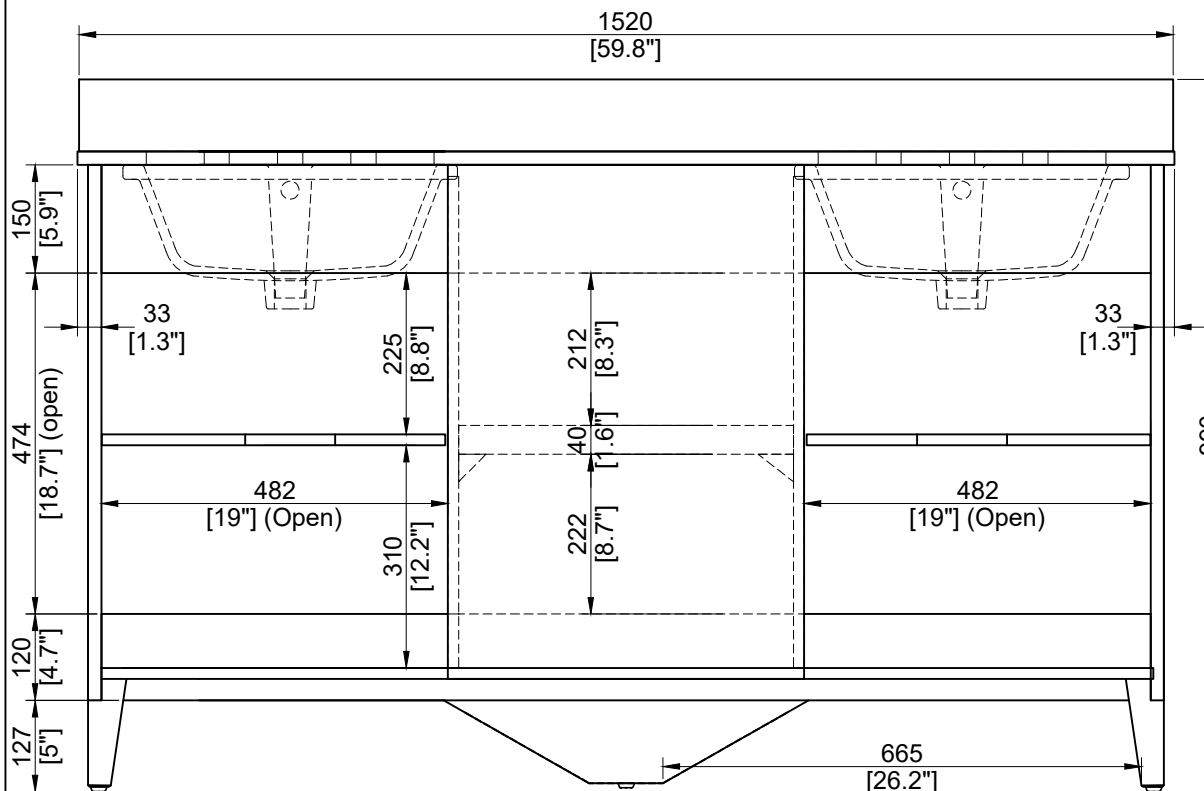
BACK VIEW
