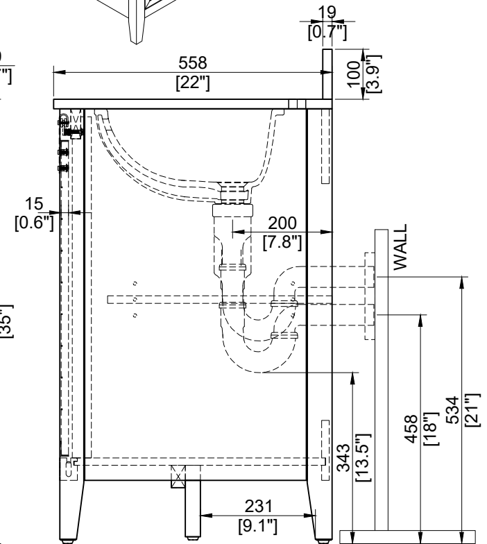
SIDE VIEW 1
