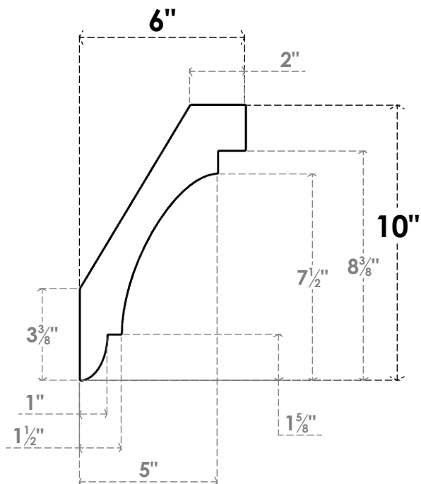
SIDE PROFILE
