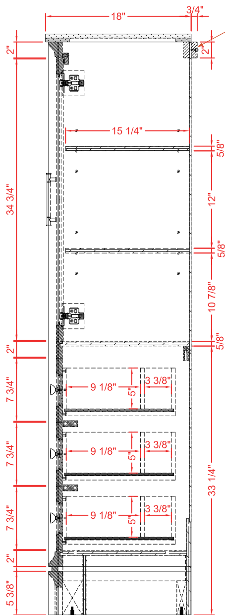
SIDE VIEW
