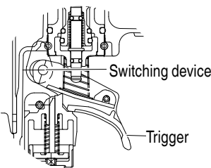
Enlarged view of the valve part
