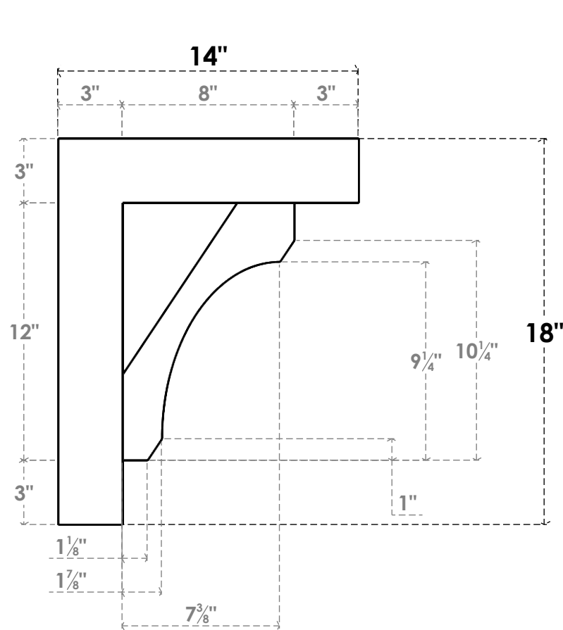
SIDE PROFILE
