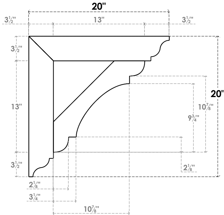
SIDE PROFILE
