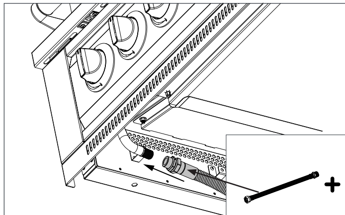
Metal Corrugated Extension Hose
