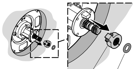
Collar/Collier/Collarín O-Ring/Joint torque/Arosello
