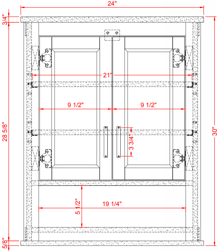
FRONT VIEW
