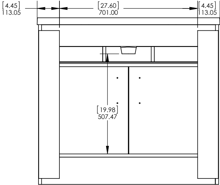
Back View / Vista Trasera
