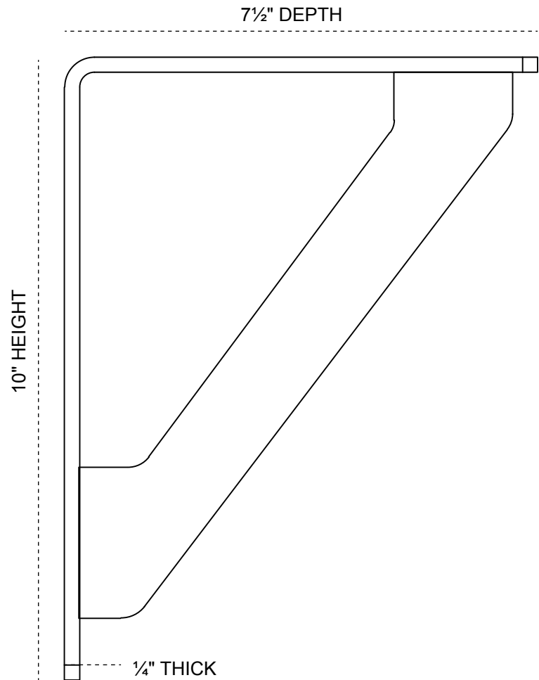
SIDE PROFILE
