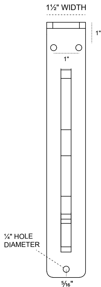
FRONT PROFILE
