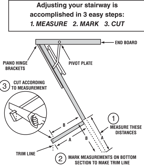
FIGURE 7A - ADJUSTMENT TO CEILING HEIGHTS
