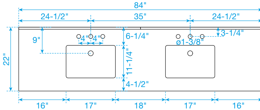
TOP VIEW OF VANITY CABINET
