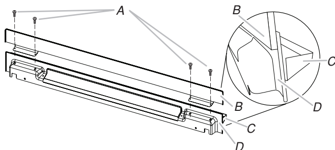
A. #8-18 x 1/4" (6.4 mm) screws B. Warming drawer deflector C. Vent D. Warming drawer deflector
