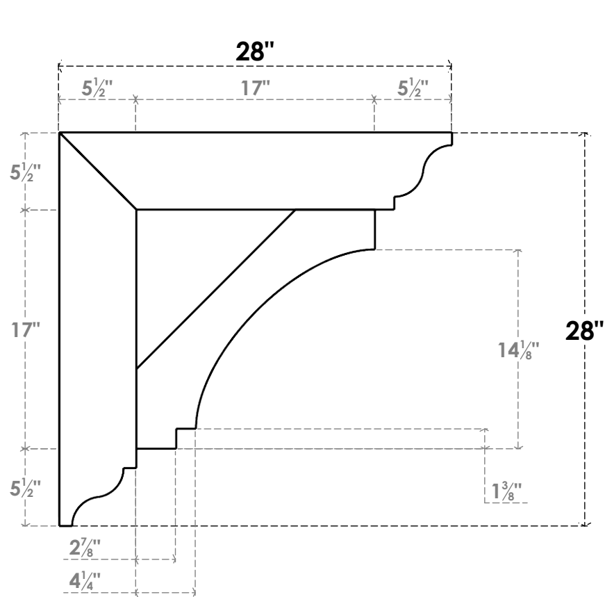
SIDE PROFILE
