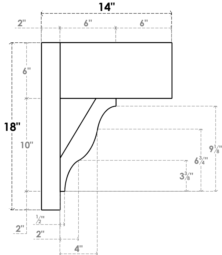
SIDE PROFILE
