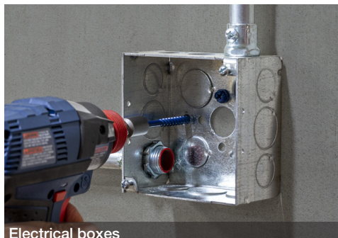
Electrical boxes
