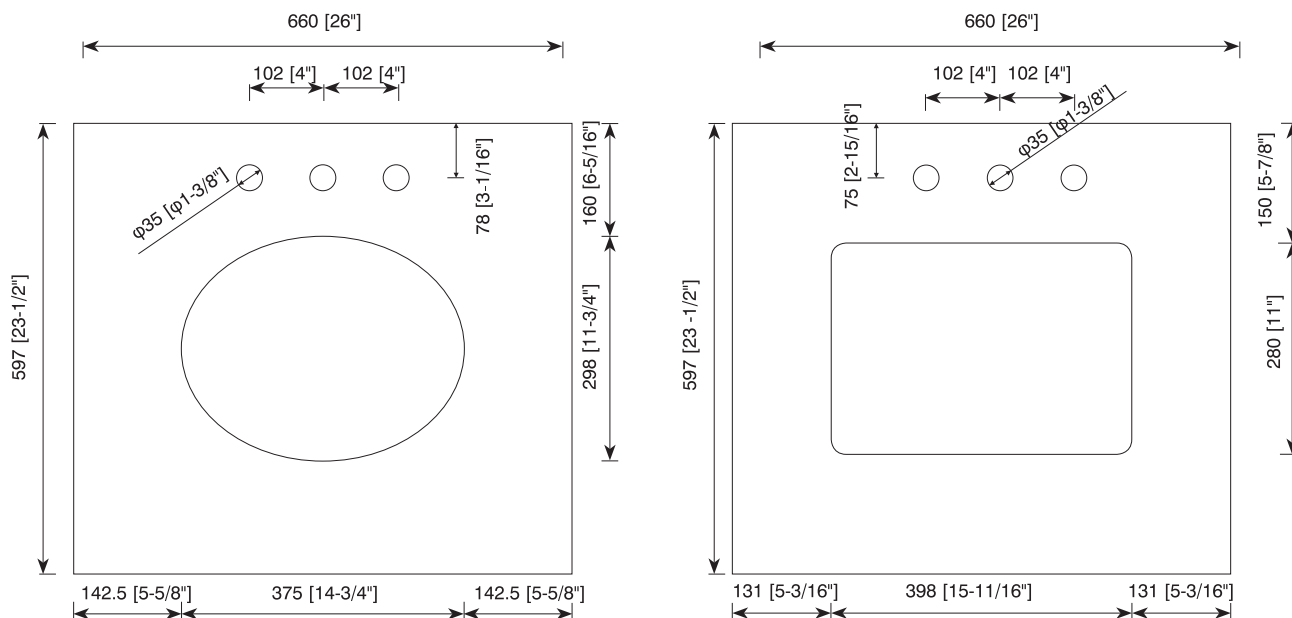
James Martin - Stone Top Measurement Specifications
