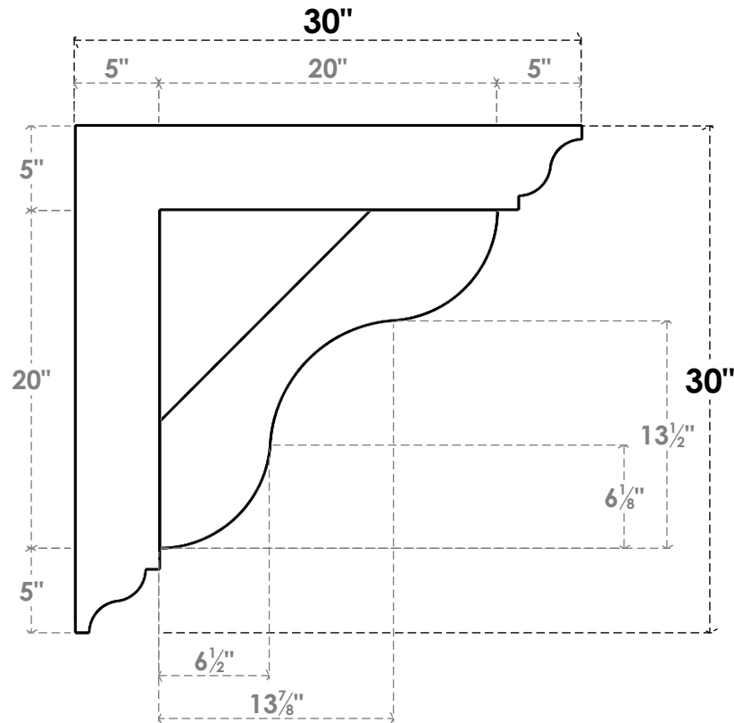
SIDE PROFILE
