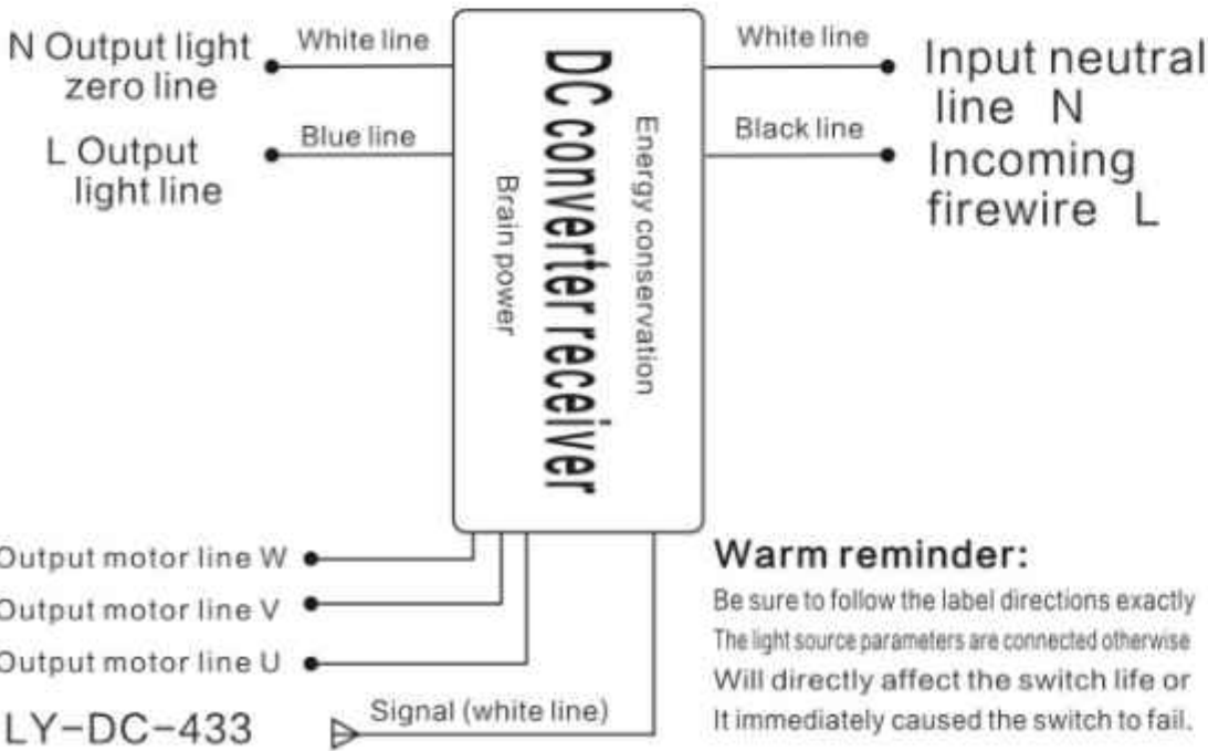
DC frequency conversion receiver wiring diagram
