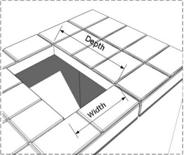
Drop-In Side Burner Cut-out Type
