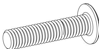
Pan Head Phillips Screw M4x23 QTY 4
