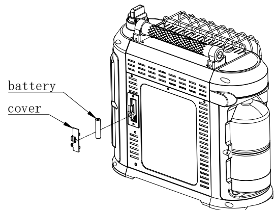
Fig. 3 - Battery location for spark module
