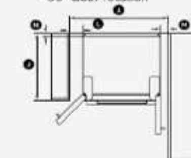
Plan View Flush with refrigerator door— 90° door rotation
