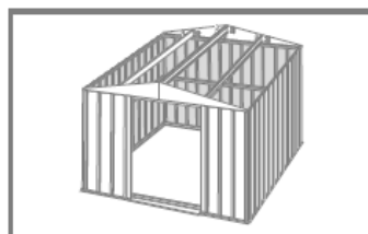
Install roof beams
