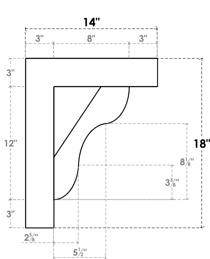
SIDE PROFILE
