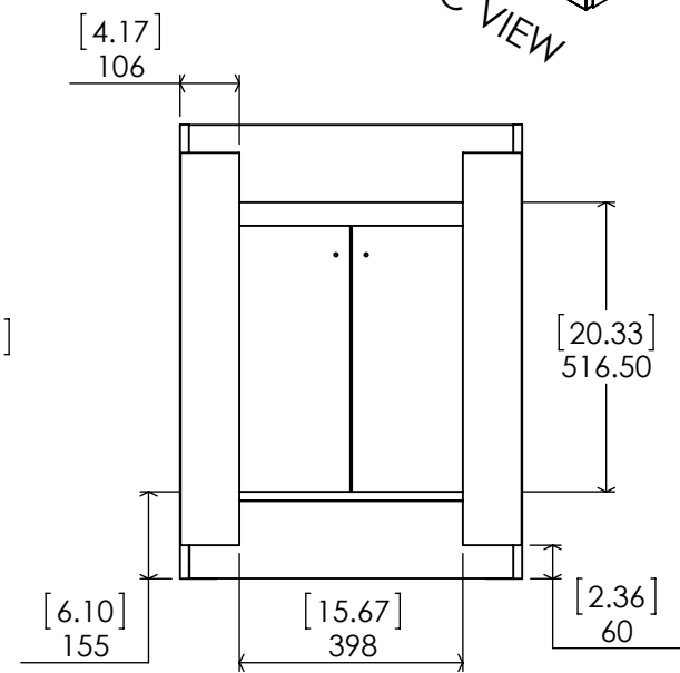
BACK VIEW
