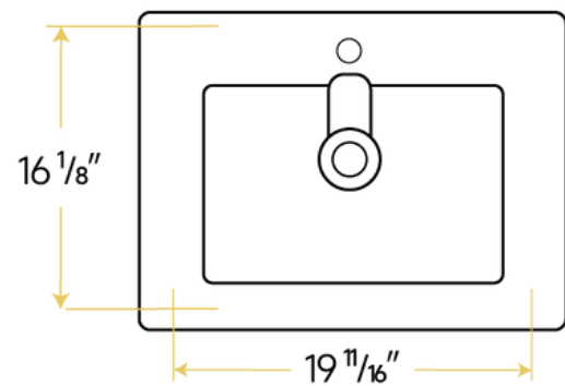
Cutout Size
