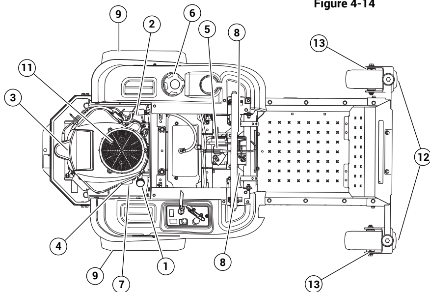
Mowers with Kawasaki engines
