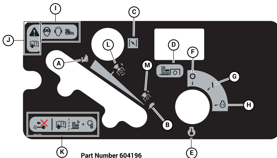
Part Number 604196
