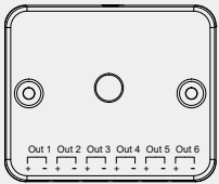
LED Receiver - TRC-H-CMO-SY
