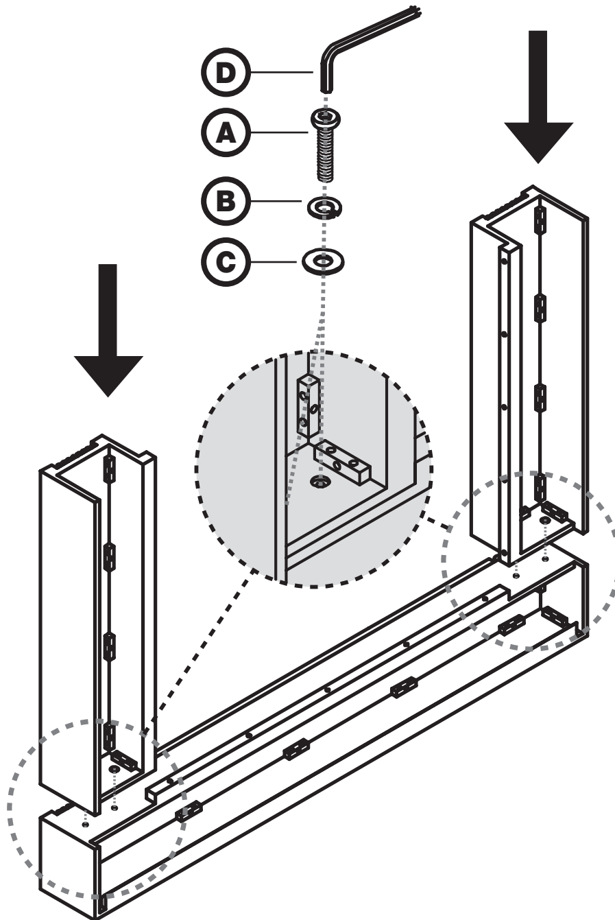
A | Bolt 1/4" x 1-3/4" | x4
