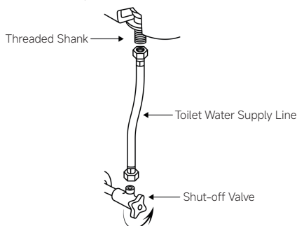
Water Supply Installation
