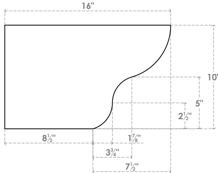
SIDE PROFILE
