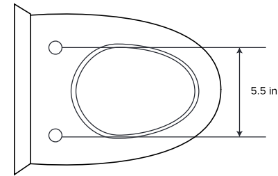
Required Distance Between Mounting Holes
