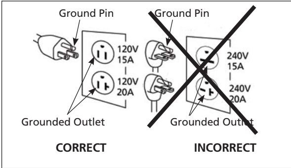
Figure 2 - Grounding Method
