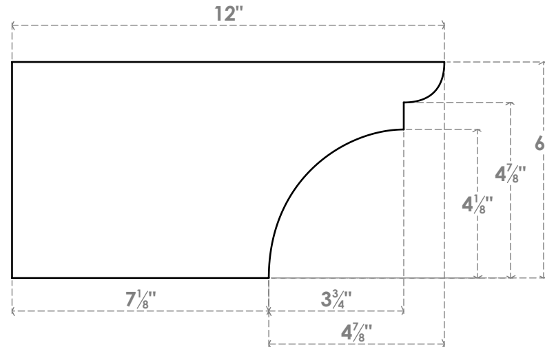
SIDE PROFILE
