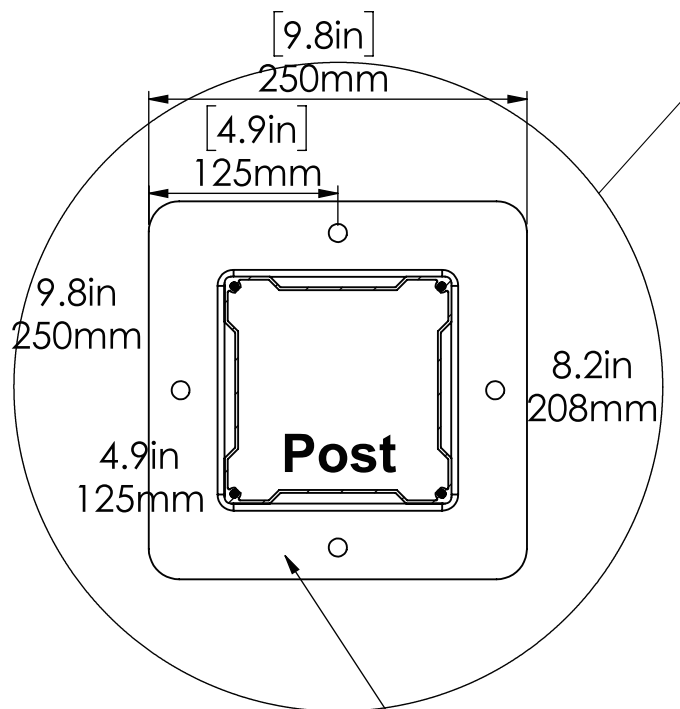
Post Mount Post Detail
