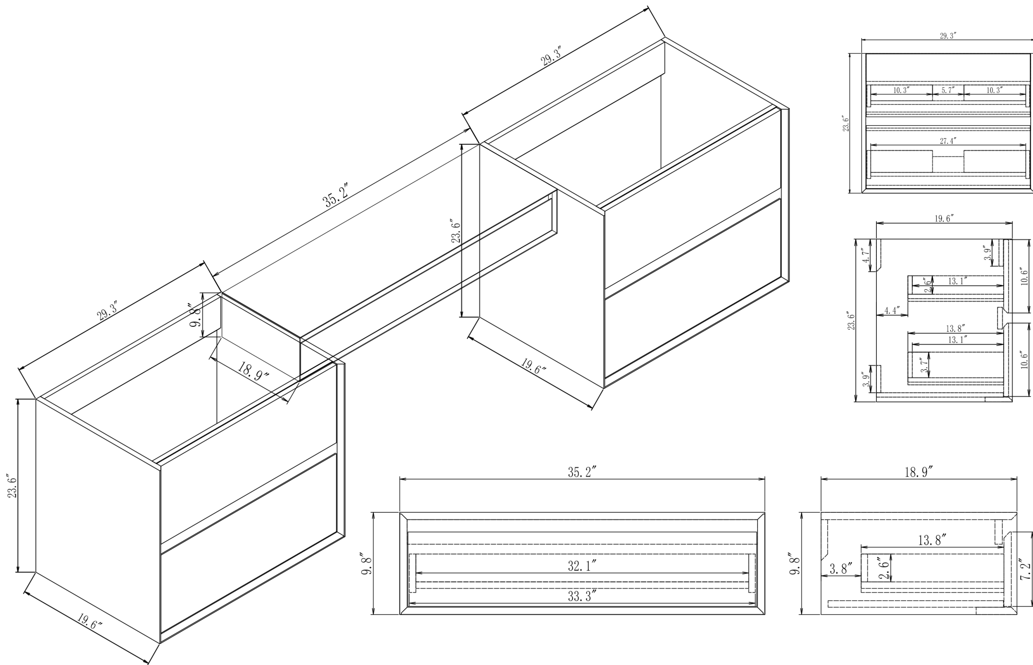
Kingdee-30+36+30 Vanity Base
