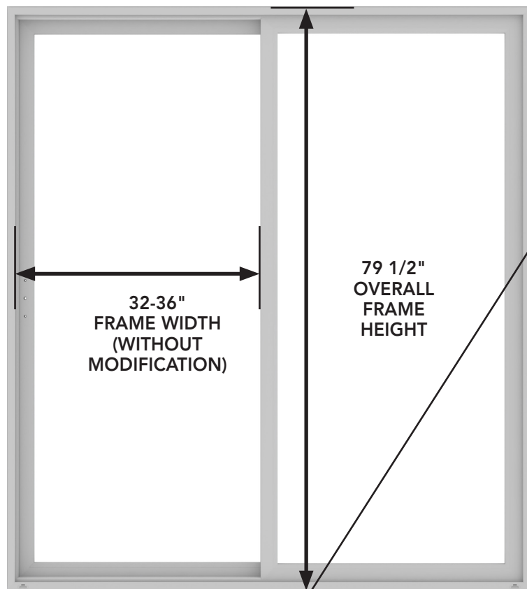
FIG. A EXTERIOR VIEW
