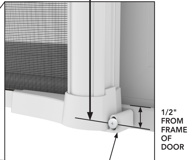
LOWER HOUSING END CAP ATTACHMENT BRACKET WITH SCREW
