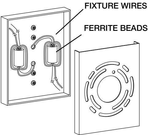
FIGURE 3 Applies only to fixtures with two modules.
