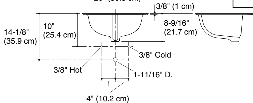
Standard Installation
