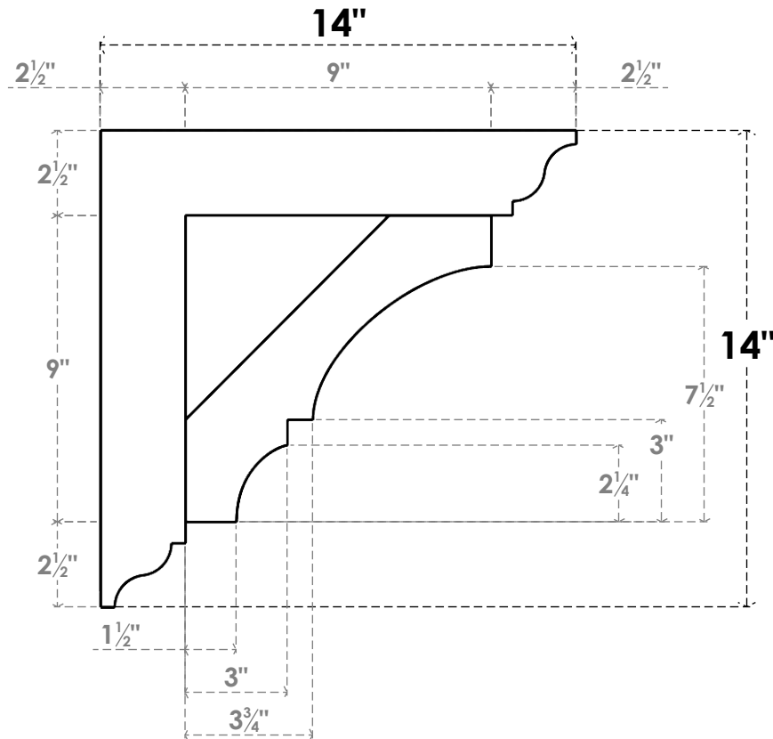
SIDE PROFILE
