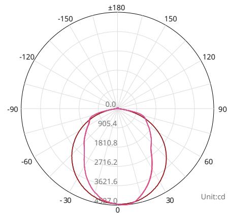
C Plane Distribution Diagram
